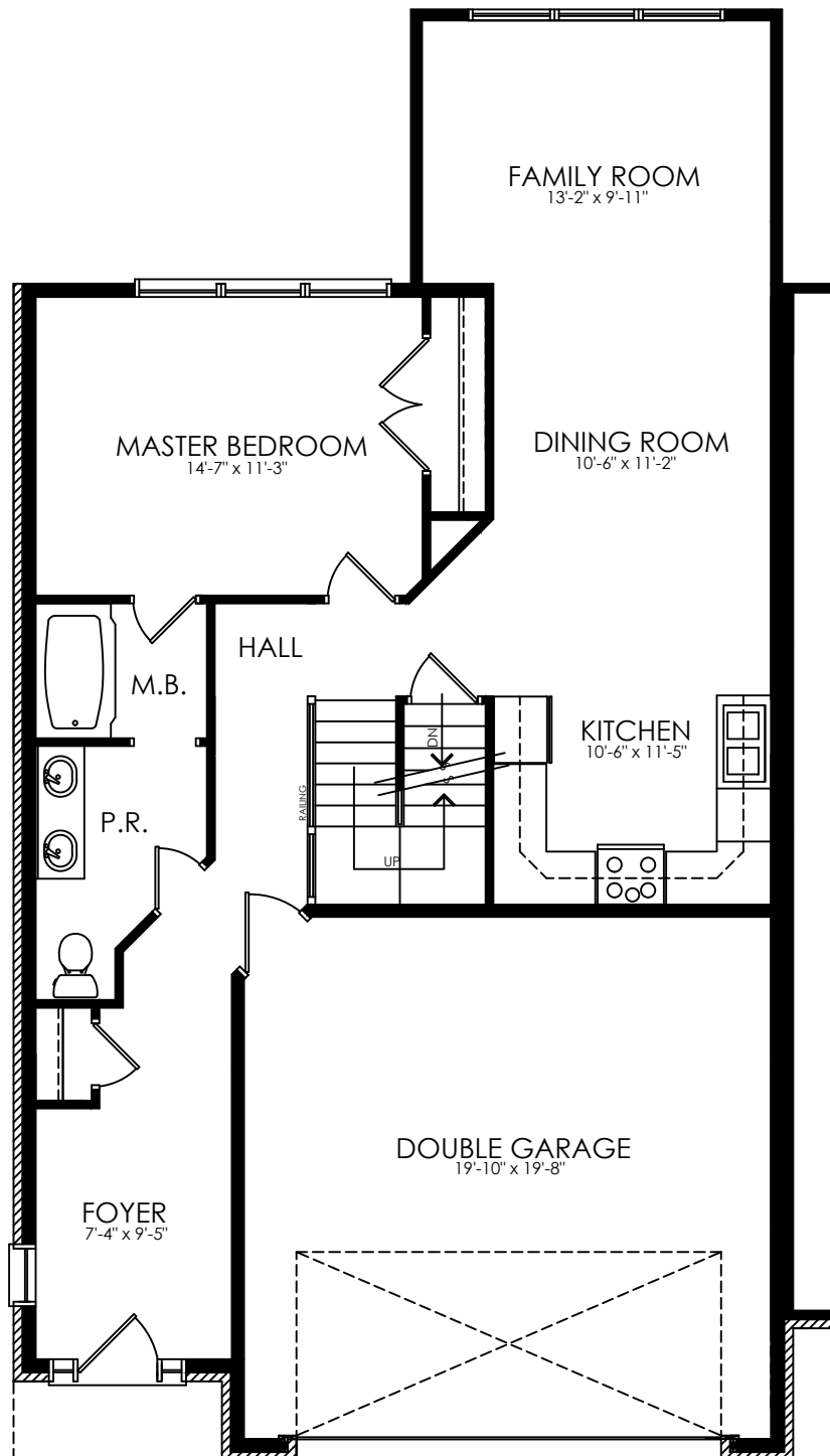
ELLISON PLACE MULBERRY & WILLOW FIRST FLOOR MASTER BEDROOM OPTION 2
